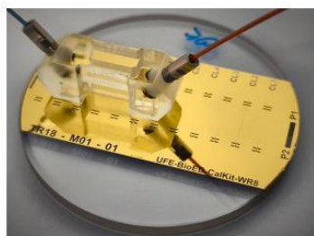
On-wafer VNA-Calibrated subTHz microfluidics
